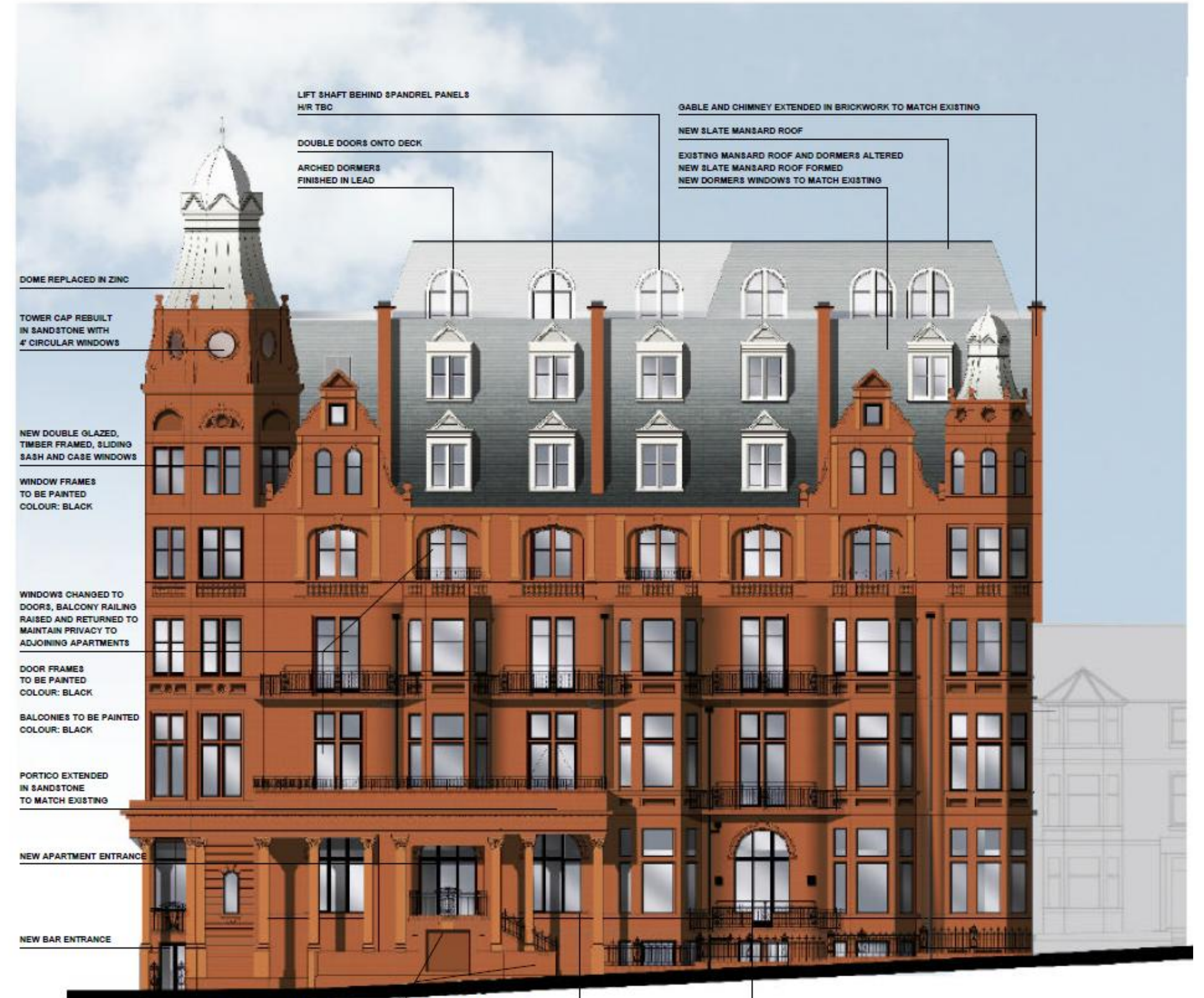
WEST ELEVATION GOLF PLACE
